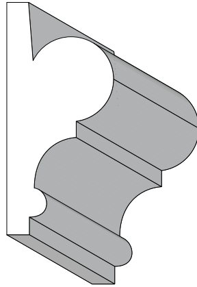
BA 1135 13/16" x 1-13/16" BA 1760 Side
