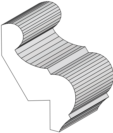
BA 511 3/4" x 2-1/16"
