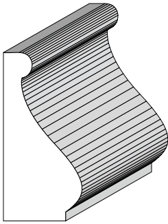
BA 525 9/16" x 1-1/4"
