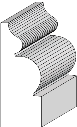
BA 782 3/4" x 1-7/8"
