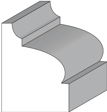
BA 1954 1-9/16" x 1-1/8"
