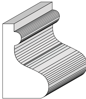
BA 557 13/16" x 1-1/4"
