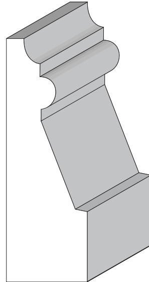
BA 1354 13/16" x 2-1/2"
