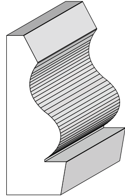
BA 22 5/8" x 1-3/4"
