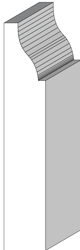
BA 506 3/4" x 4"
