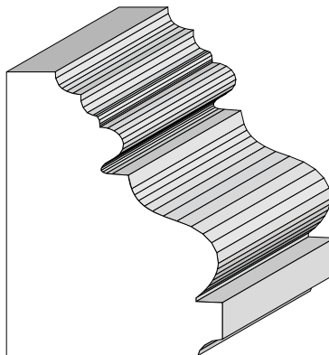
BA 672 1-1/4" x 1-5/8"
