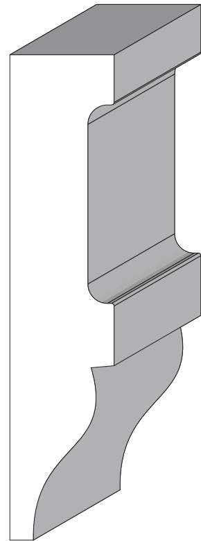
BA 1857 13/16" x 3-5/8"
