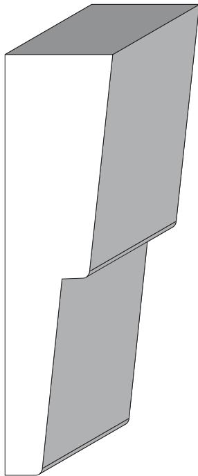
BA 1959 13/16" x 3-3/16"
