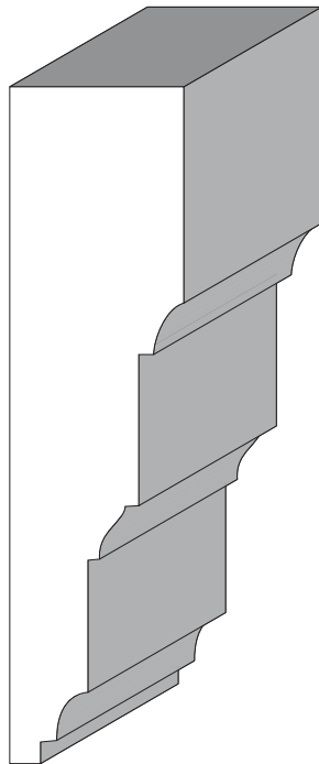
BA 2006 13/16" x 3-3/16"
